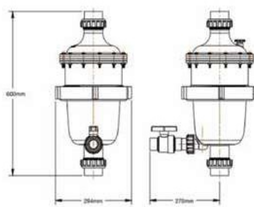
Multicyclone 16 Peso 7 kg
