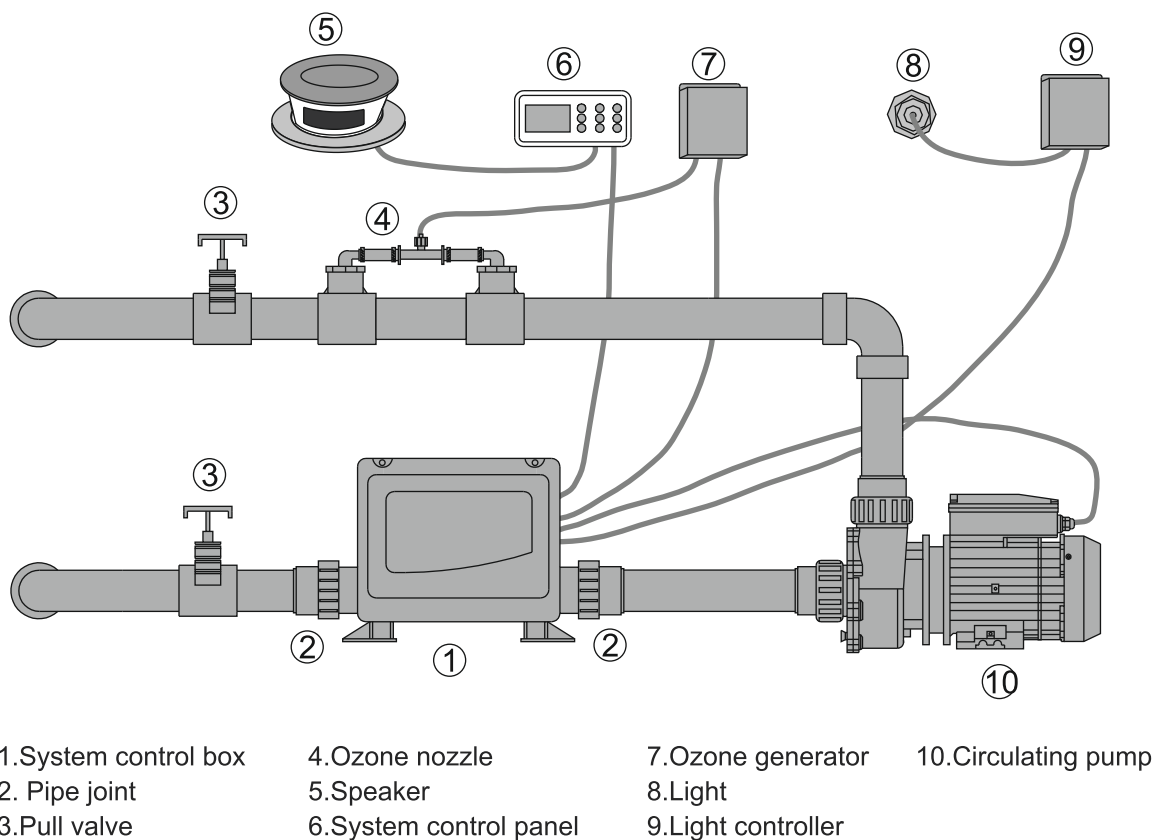
Side view of control device
