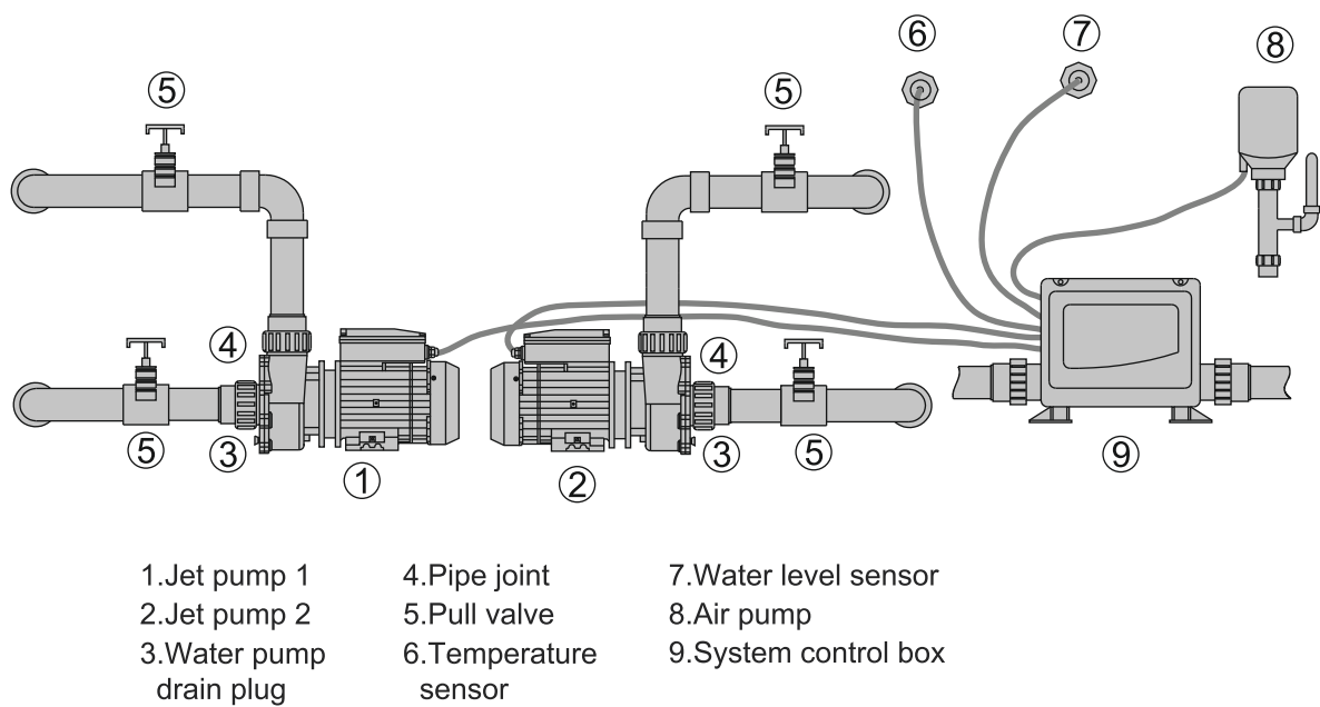
Side view of jet pump
